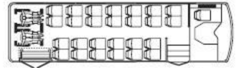
618 • 26-passenger, two-wheelchair, rear lift
