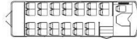
605 • 26-passenger, rear luggage
