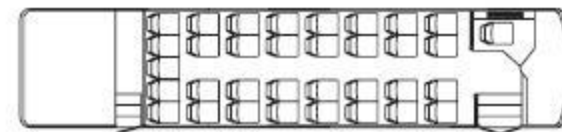
704 • 33-passenger, rear luggage
