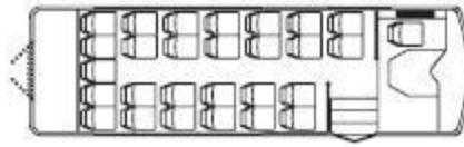
601 • 27-passenger, rear luggage
