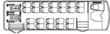
606 • 24-passenger, two-wheelchair, rear lift
