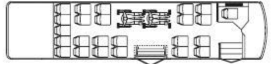
702 • 23-passenger, two-wheelchair, mid-body lift
