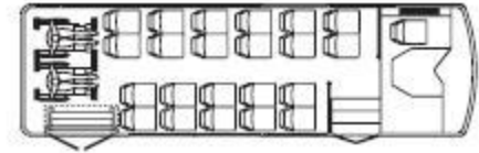
602 • 22-passenger, two-wheelchair, rear lift
